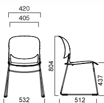
OUTLINE 610 SKID
