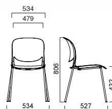
OUTLINE 610 4 LEG
