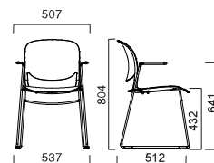
OUTLINE 610 SKID WITH ARMS
